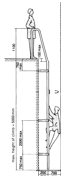
⑫ Fixed catladder
